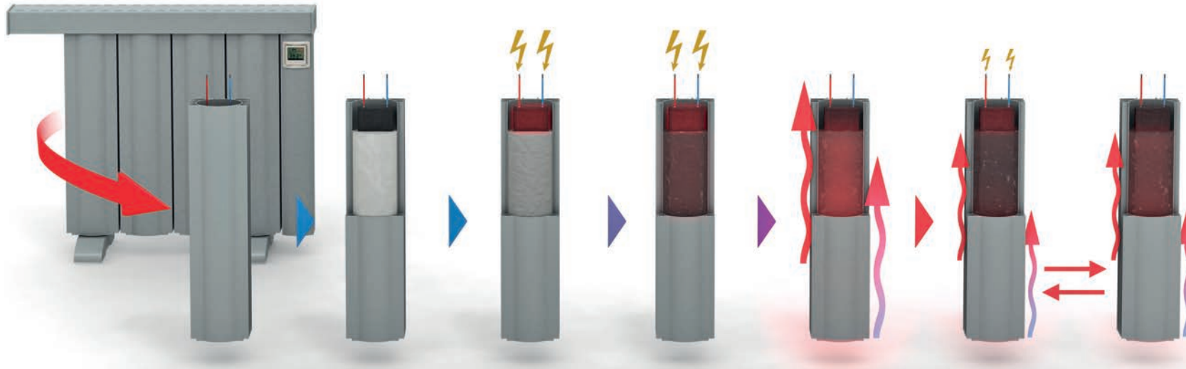
"Mini-power station" in the heater: The phase change material changes its aggregate state depending on the heat energy supplied and the ambient temperature for the optimal storage and release of heat.
